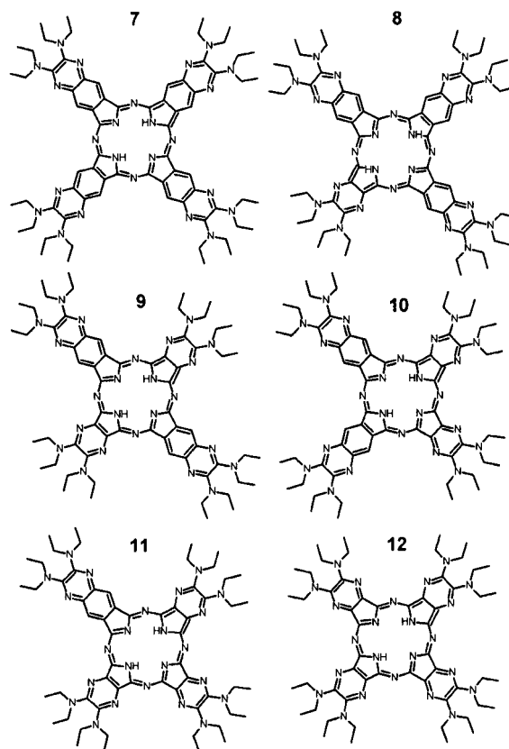
Figure 2. Structures of the PQPs in the reaction mixture.
