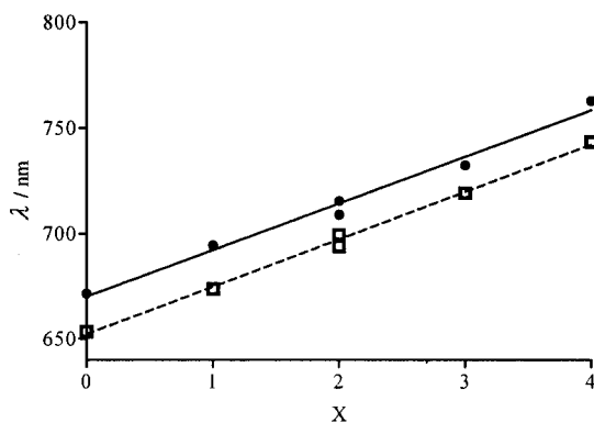
Figure 5. The Q-band absorption centres of H 2 P 4-x Q x P (●) and Zn P 4-x Q x P (□), (x = 0–4) vs. x, the number of inserted benzene rings into the macrocycle.
