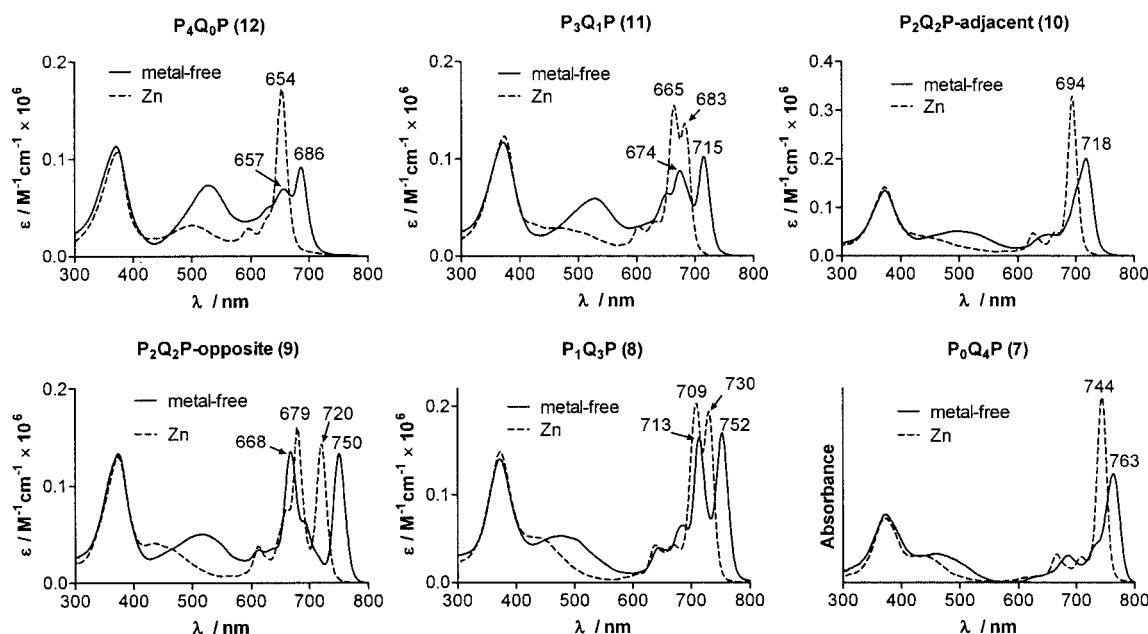
Figure 4. UV/Vis spectra of metal-free PQPs in dichloromethane and zinc PQPs in THF.
