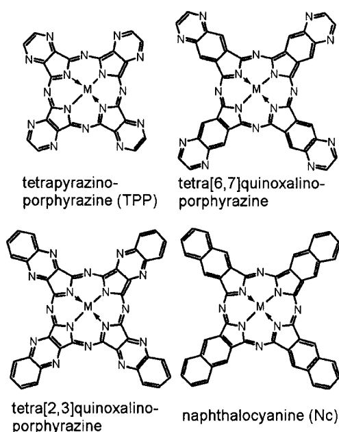
Figure 1. General structures of macrocycles discussed in this work.
