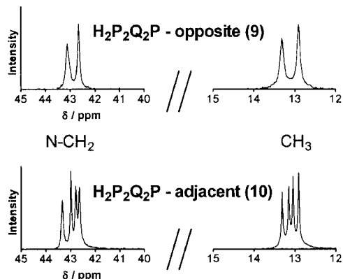
Figure 3. ^{13}\text{C} NMR spectra of the peripheral diethylamino groups of 9 (opposite) and 10 (adjacent).
