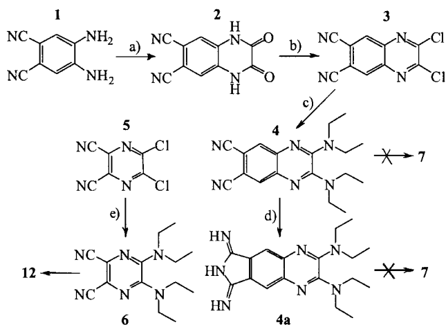
Scheme 1. Synthetic strategy. Reagents and conditions: a) EtOH, diethyl oxalate, 140 °C, 8 h; b) 1,2-dichloroethane, SOCl 2 , DMF, reflux, 3 h; c) diethylamine, THF, room temp., overnight; d) NH 3 , butanol, 90 °C, 30 min; e) diethylamine, THF, reflux, 6 h.
